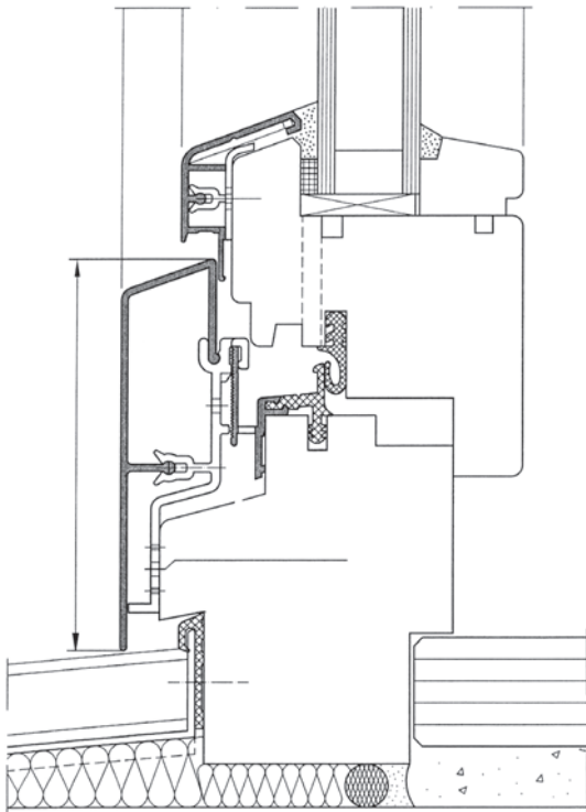
Profile of a timber window with aluminium cladding
